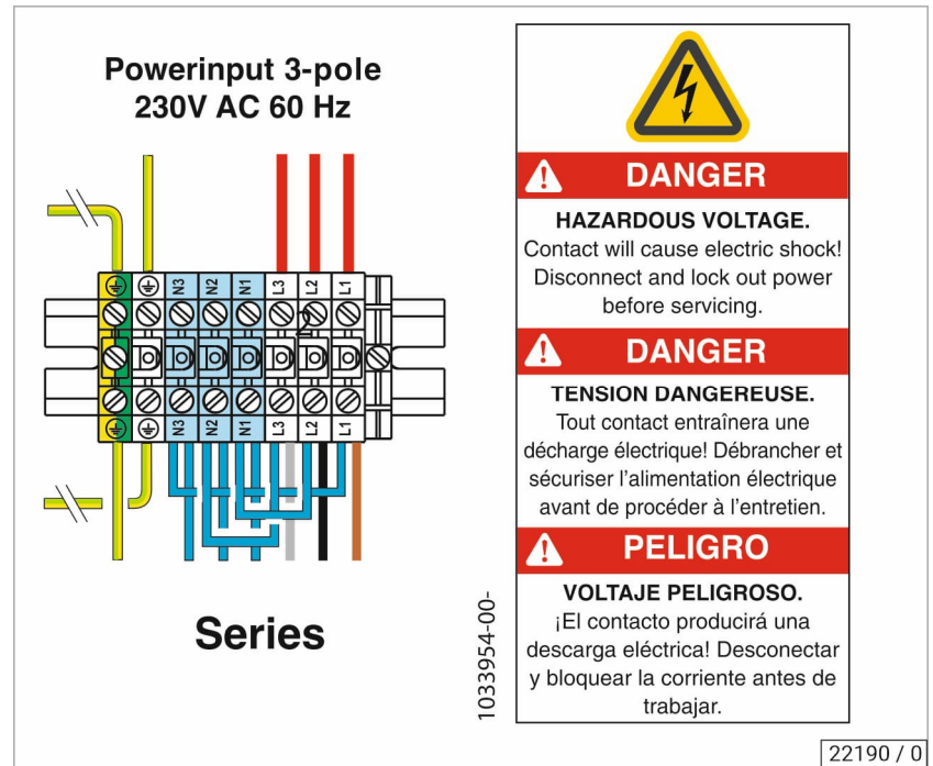
14: USA mains connection sticker (1033954-..)
